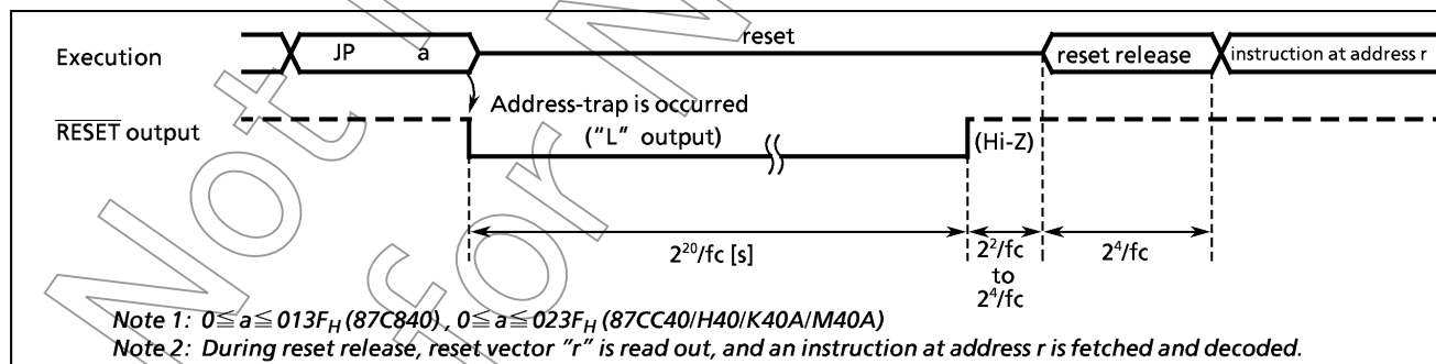
Figure 1-31. Address-Trap-Reset
