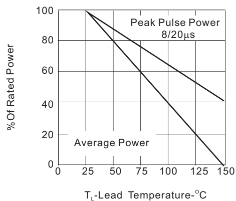
FIG. 2-Power Derating Curve
