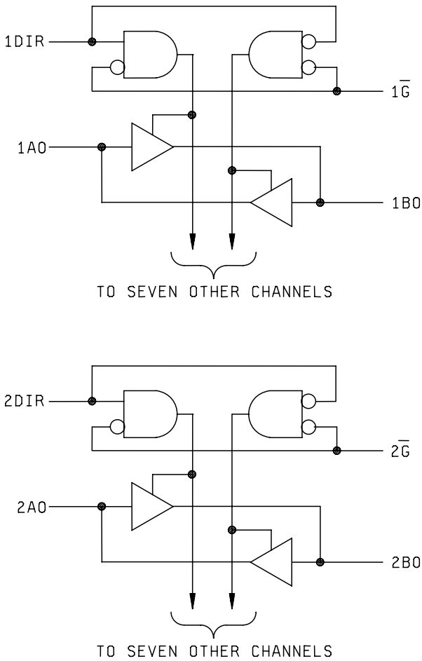
FIGURE 4. Logic diagram.
