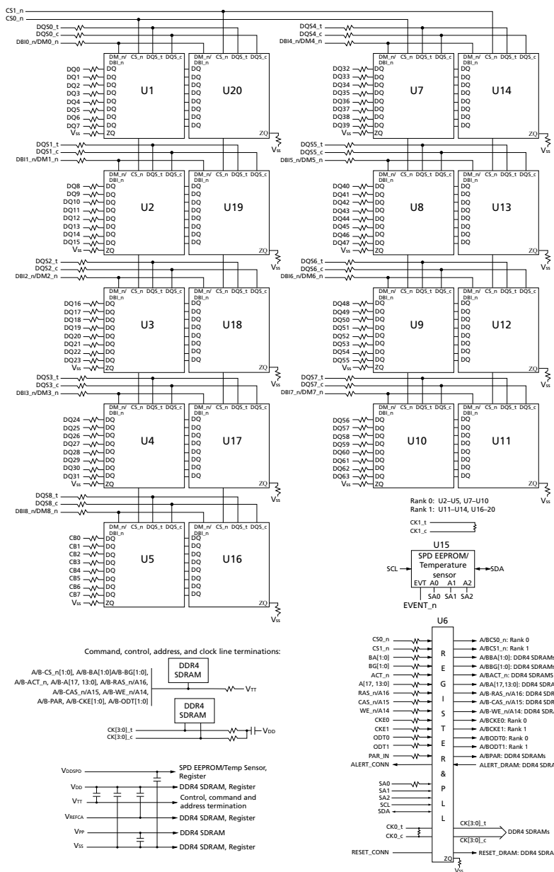
Figure 3: Functional Block Diagram, R/C-H (PCB 2050)
