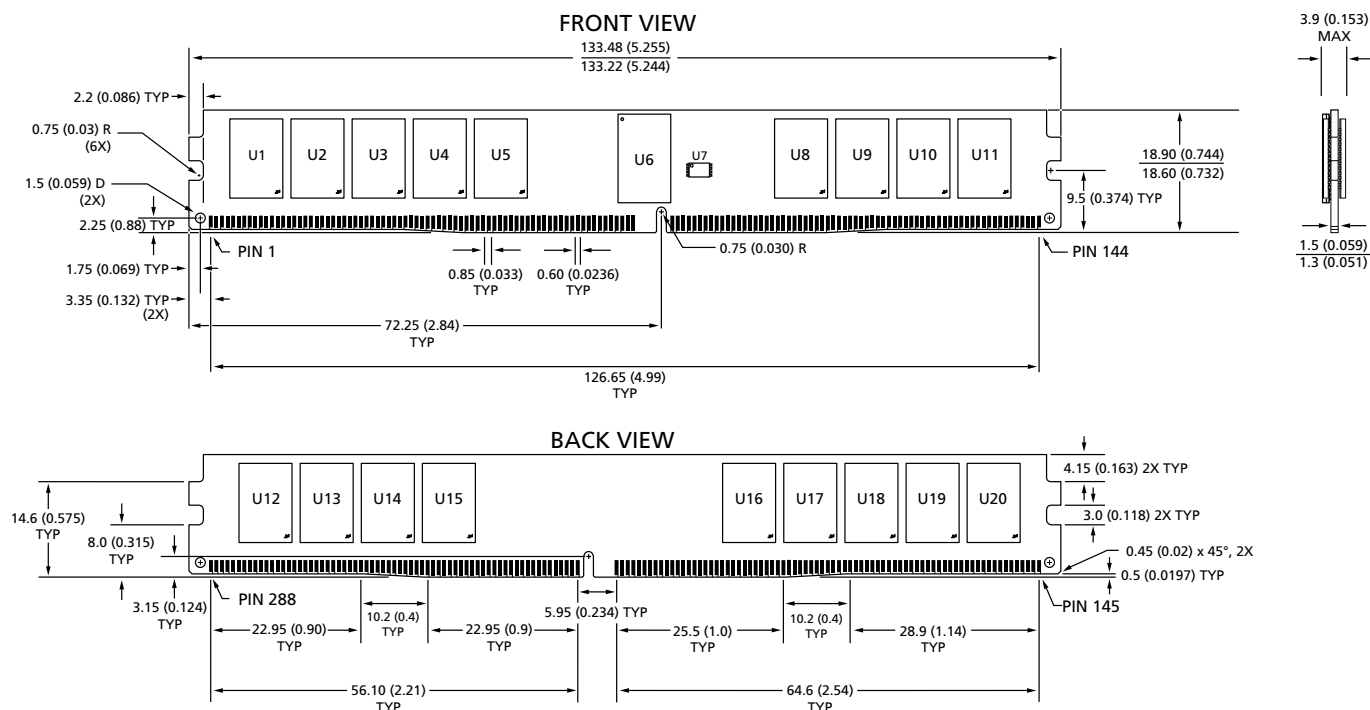
Figure 6: 288-Pin DDR4 RDIMM, R/C-H1 (PCB 2582)
