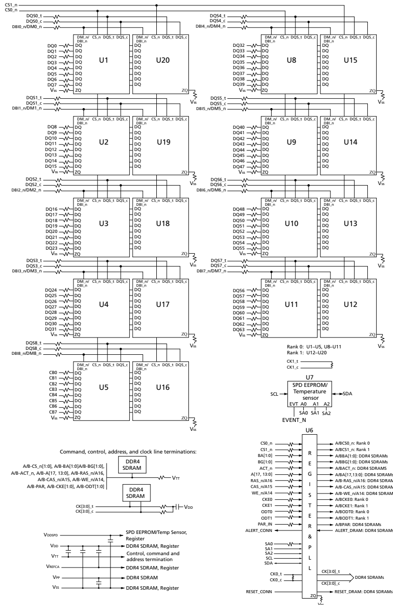
Figure 4: Functional Block Diagram, R/C-H1 (PCB 2582)
