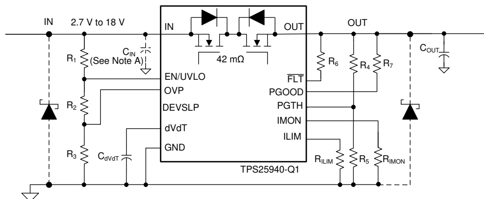
Figure 11-1. Circuit Implementation with Optional Protection Components
