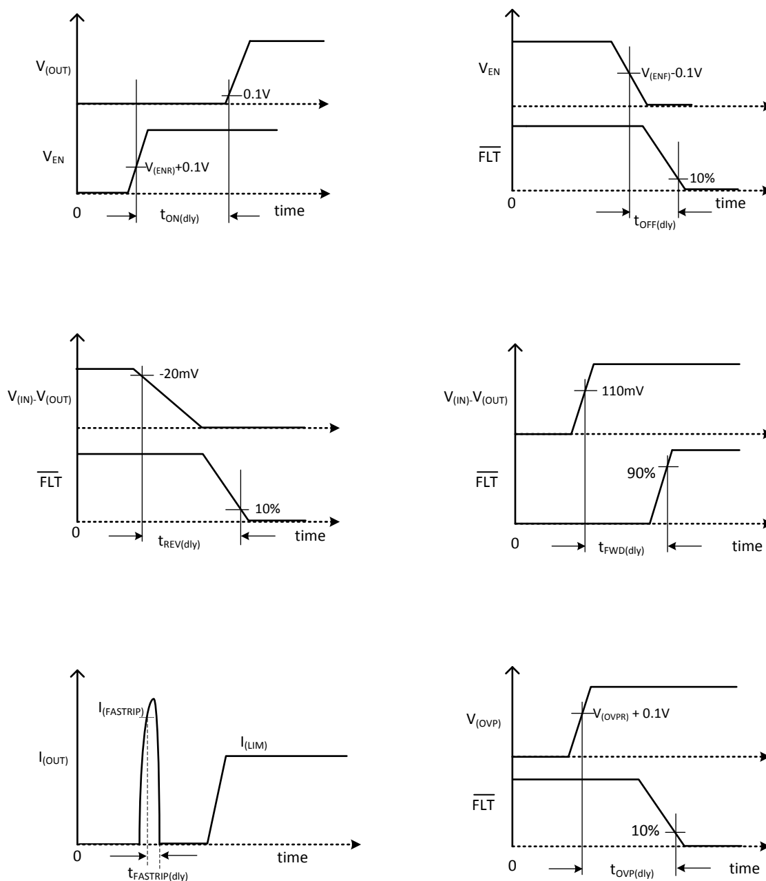
Figure 8-1. Timing Diagrams
