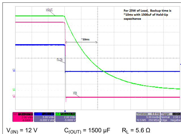
Figure 10-24. Hot-Plug Out Condition
