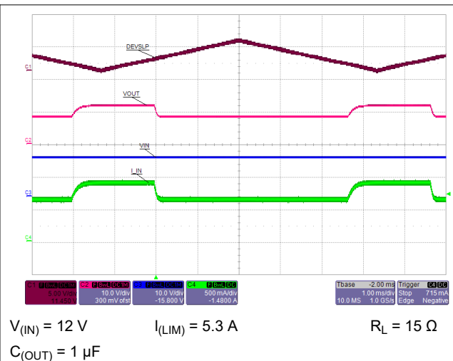
Figure 9-5. IN and OUT of DevSleep Mode with 800-mA Load. In DevSleep, Load Current Gets Limited to I_{(\text{DEVSLP}(\text{LIM}))}
