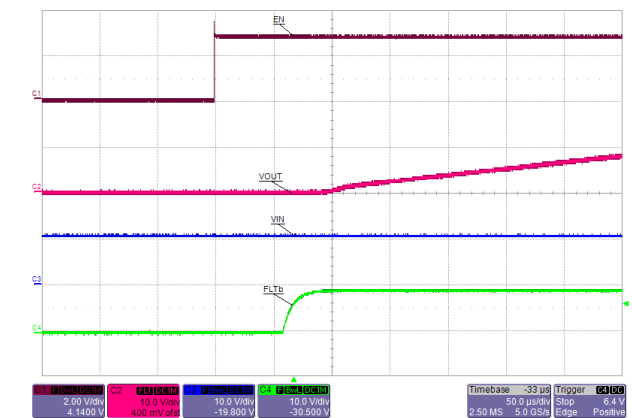
Figure 7-32. Turn ON with Enable
