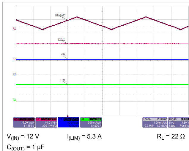
Figure 9-4. IN and OUT of DevSleep Mode with 550-mA Load
