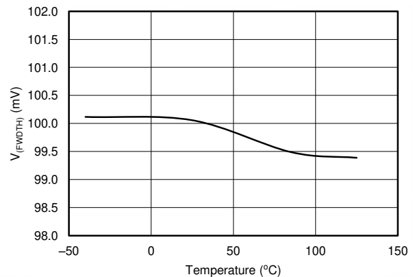
Figure 7-30. V_{(\text{FWDTHT})} vs Temperature
