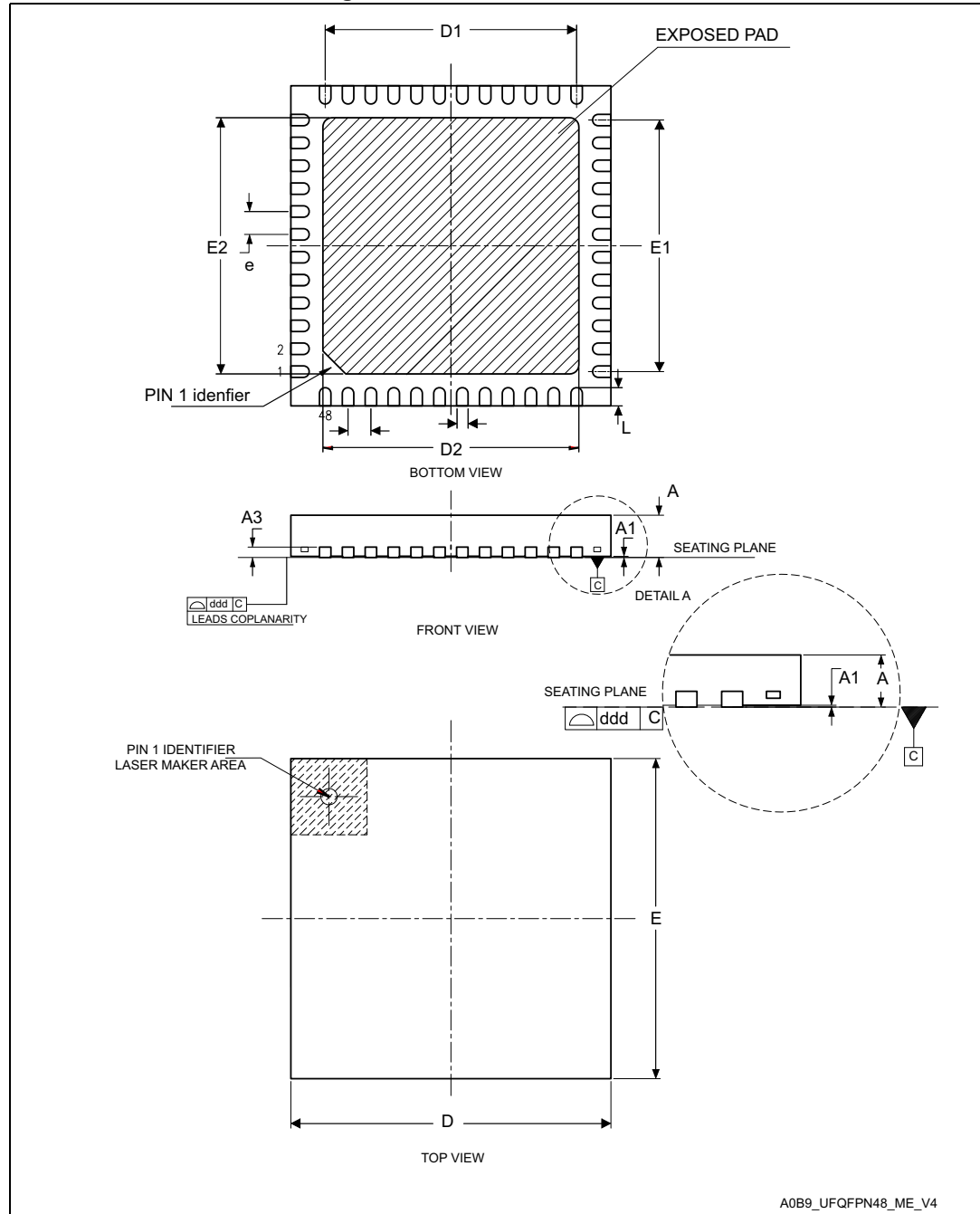
Figure 67. UFQFPN48 – Outline
