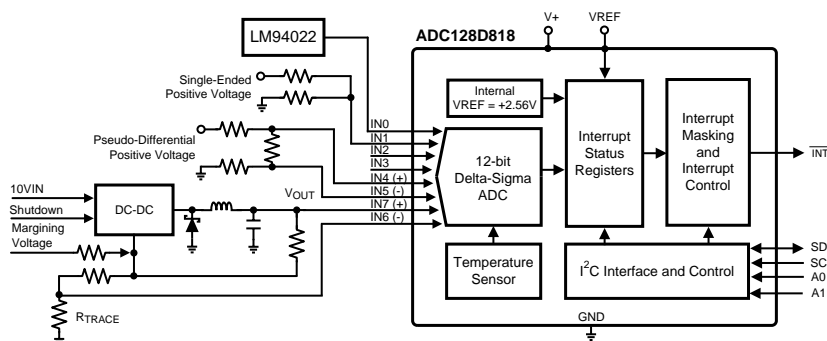
Typical Application Diagram
