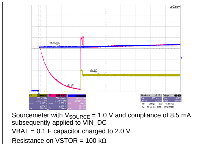
Figure 25. Startup by Battery Attach With Almost Depleted Storage Element
