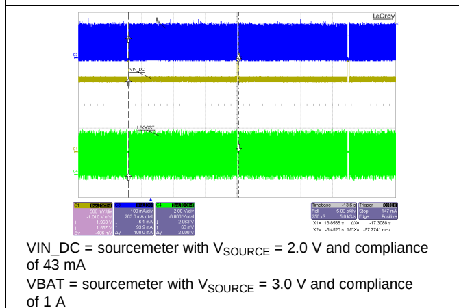
Figure 27. MPPT Operation
