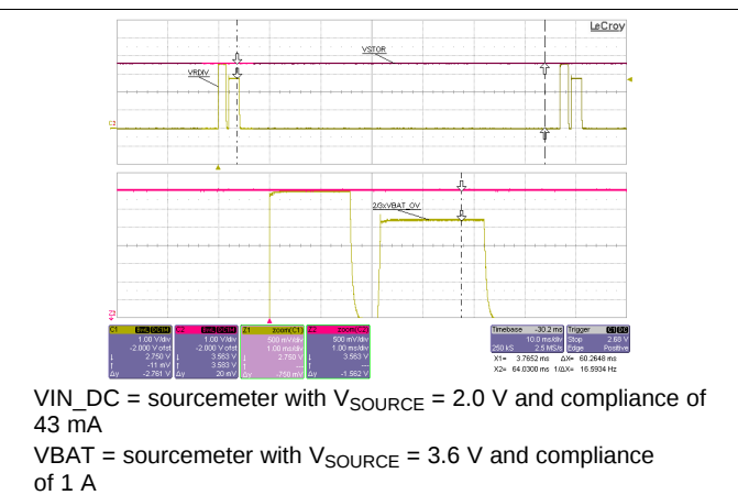
Figure 28. VRDIV Waveform
