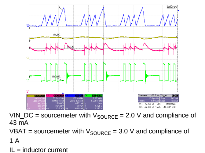
Figure 26. Boost Charger Operational Waveforms
