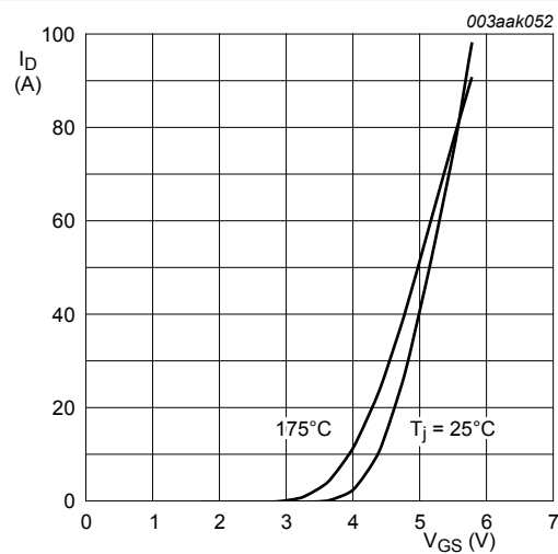
Fig. 7. Transfer characteristics; drain current as a function of gate-source voltage; typical values V DS = 10V
