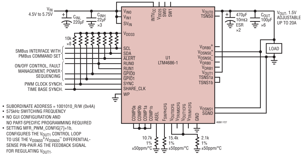
Figure 27. 20A, 1.5V Output DC/DC µModule Regulator with I 2 C/SMBus/PMBus Serial Interface
