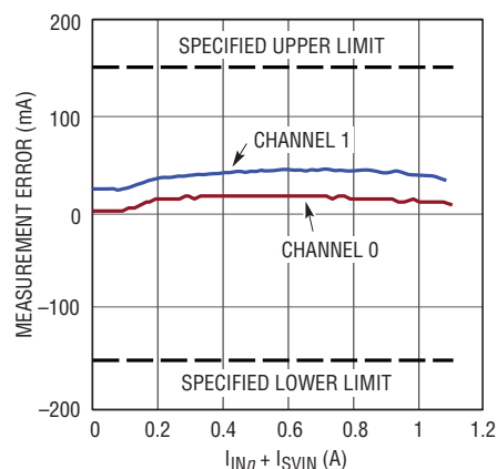
MFR_READ_IIN _n (Input Current Readback) Error vs (\text{I}_{\text{VIN}} + \text{I}_{\text{SVIN}}) , \text{MFR\_PWM\_MODE}n[0] = 1\text{b} , \text{I}_{\text{OUT}n} Swept from 0\text{A} to 10\text{A} , One Channel at a Time, \text{RUN}1-n = 0\text{V}
