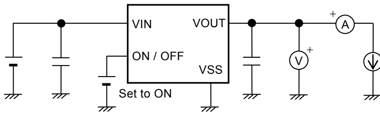
Figure 5 Test Circuit 1
