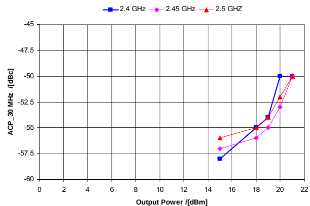
Figure 4 – ACP Data with 54MB/s 64 QAM OFDM
