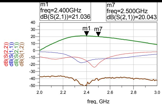
Figure 6 – S-Parameter Data
