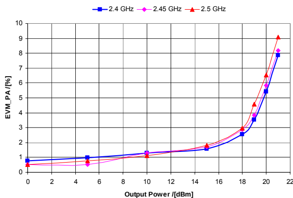
Figure 3 – EVM Data with 54Mb/s 64 QAM OFDM
