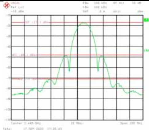
Figure 5 – Spectrum with 23dBm 11Mb/s CCK
