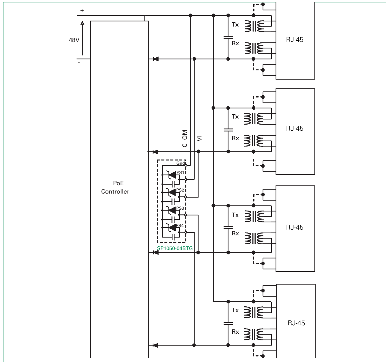
Figure 1: Typical application circuit with fully integrated PSE controller
