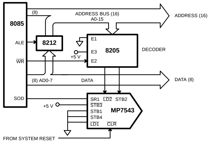
Figure 1. MP7543 8085 Interface
