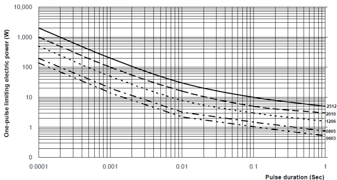
Maximum permissible peak pulse power as a function of pulse duration
