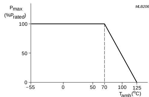
Fig. 6-1 Maximum dissipation ( P_{max} ) in percentage of rated power as a function of the operating ambient temperature ( T_{amb} )
