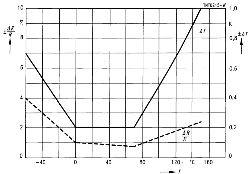
Resistance and temperature tolerances versus temperature ( \Delta T = 0,5 \text{ K} )
