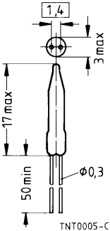
Dimensions in mm Approx. weight 0,3 g
