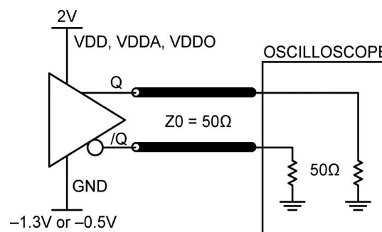
Figure 7. LVPECL Output Load and Test Circuit
