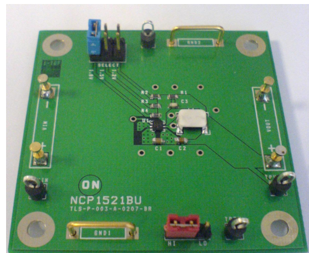
Figure 2. Board Picture in \mu DFN-6
