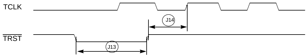
Figure 31. \overline{\text{TRST}} Timing
