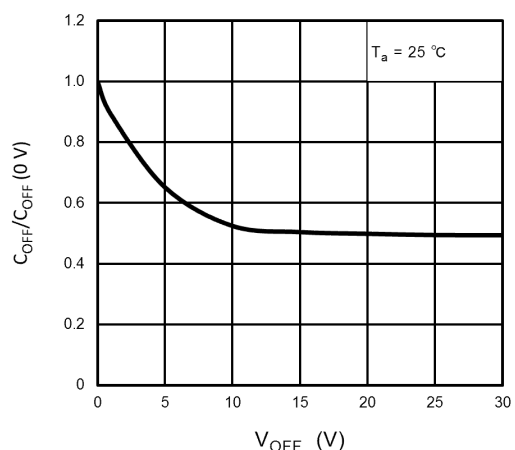
Fig. 12.11 C_{OFF}/C_{OFF} - V_{OFF}
