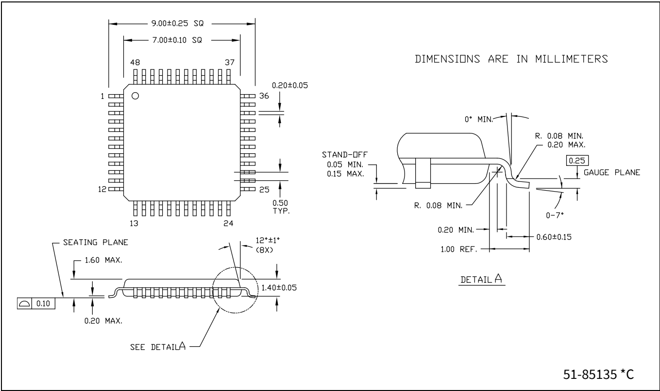
Figure 6 48LD TQFP 7x7x1.4 mm A48, PACKAGE OUTLINE, (PG-TQFP-48)
