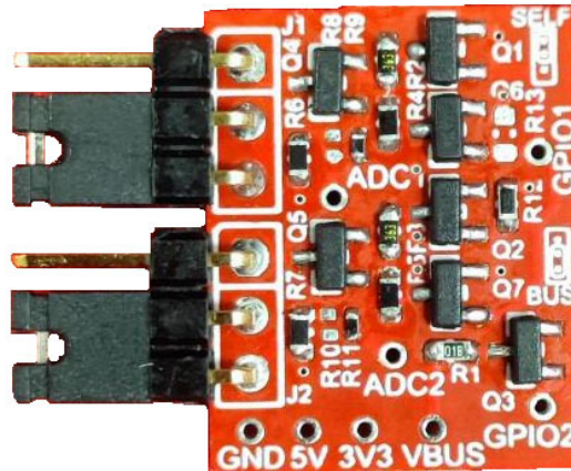
Figure 4-8. Example of Bus-Powered Configuration
