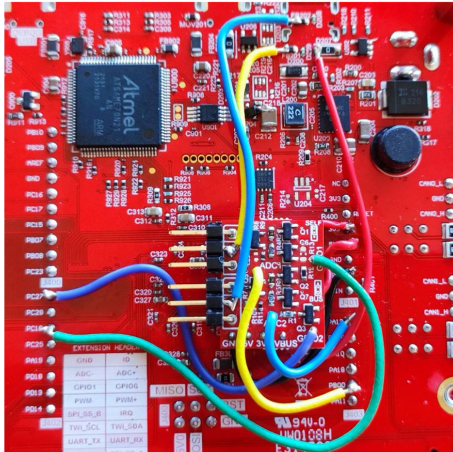
Figure 4-6. Connection Details
