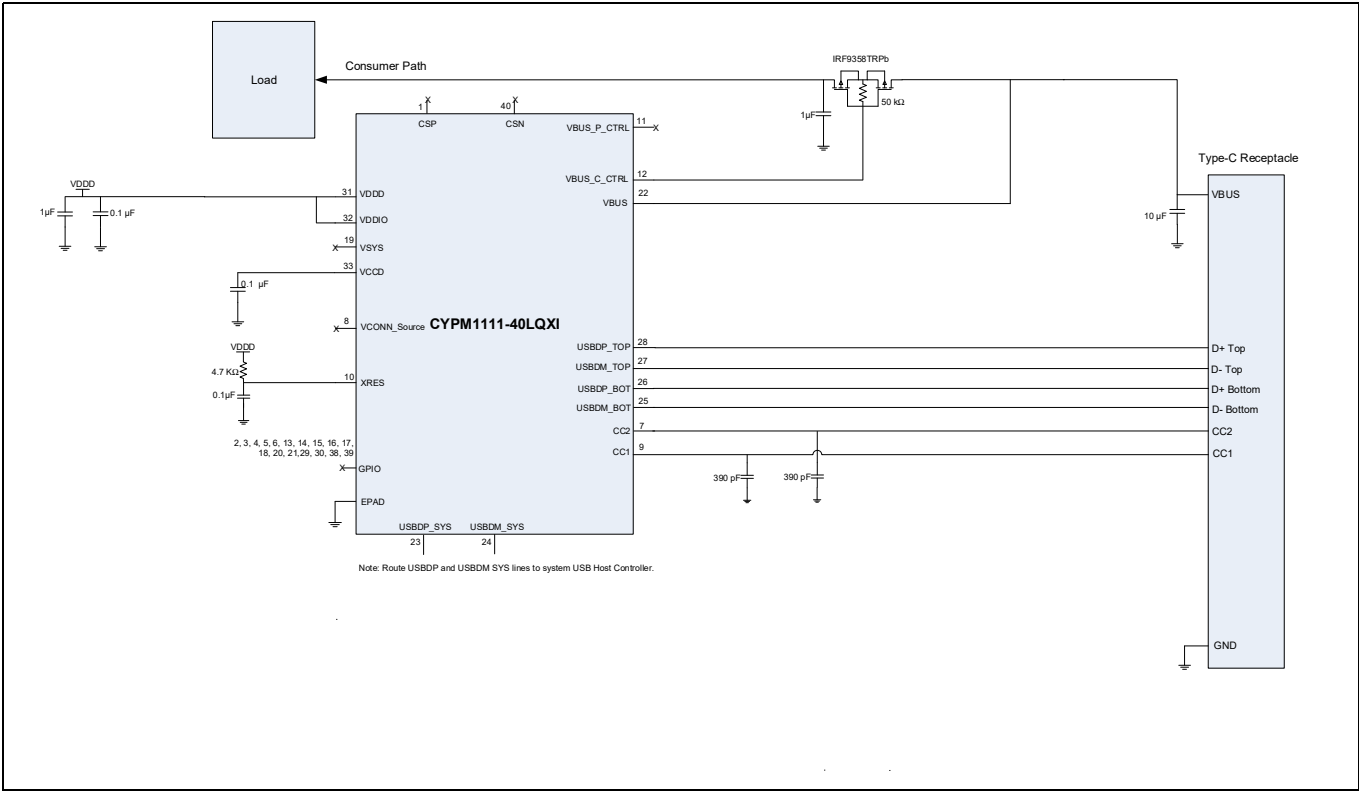
Figure 8 EZ-PD™ PMG1-S1 based sink application diagram
