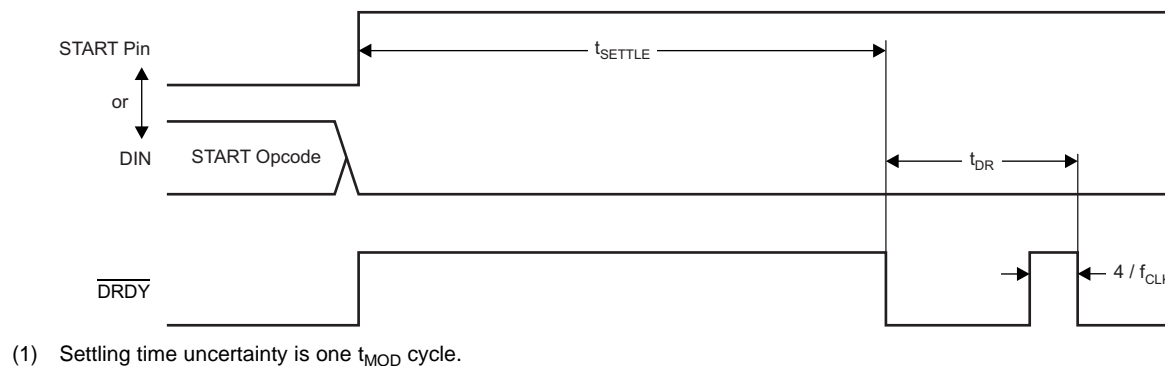
Figure 48. Settling Time
