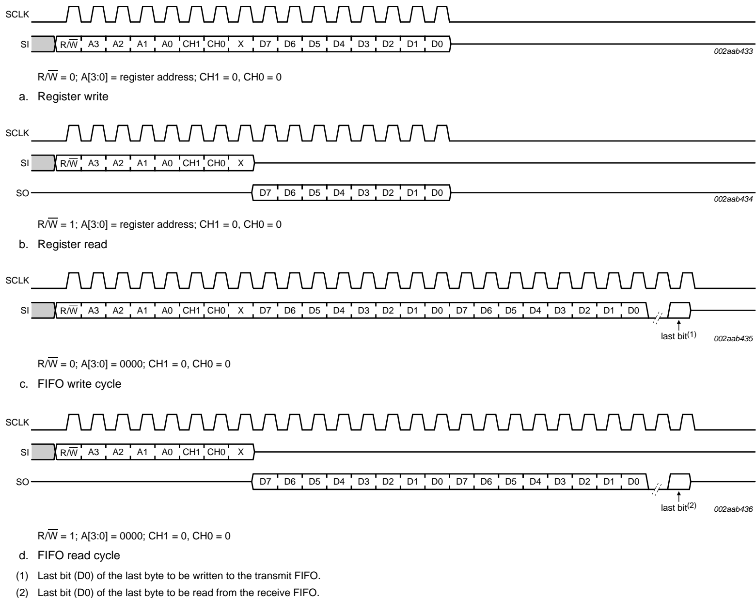
Fig 25. SPI operation
