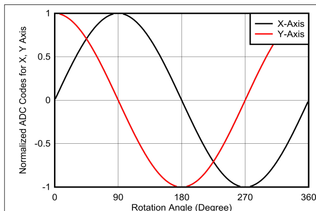
Figure 7-17. X and Y Sensor Data for Full 360 Degree Rotation for On-Axis Measurement
