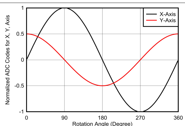
Figure 7-18. X and Y Sensor Data for Full 360 Degree Rotation for Off-Axis Measurement
