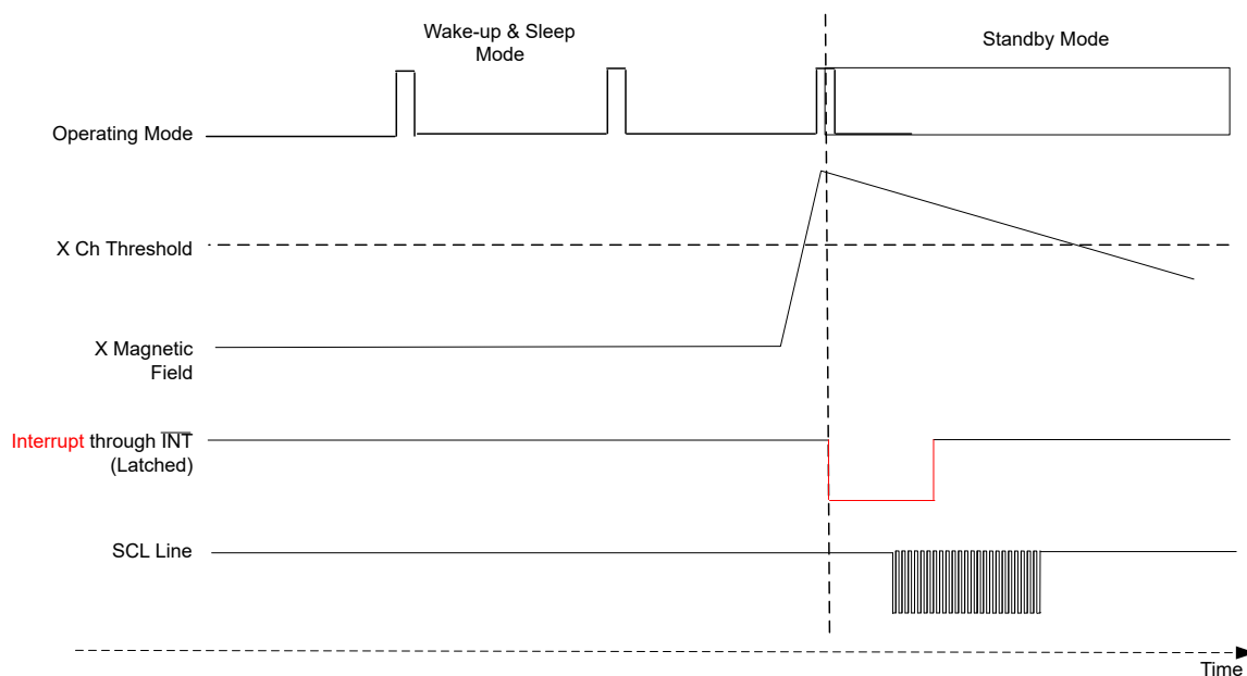
Figure 6-5. Latched Interrupt Through \overline{\text{INT}}
