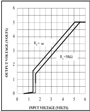
Dropout Characteristics
