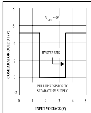
Error Comparator Output
