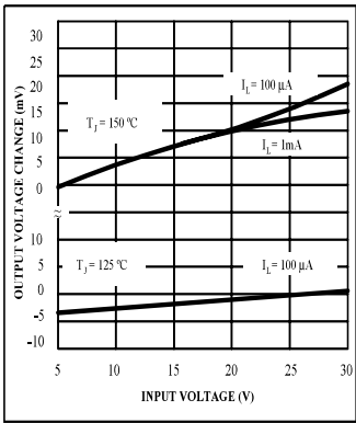
Line Regulation
