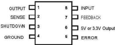
8-Pin Surface Mount (S)
