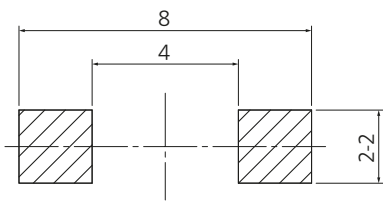
PWB land pattern for reference
