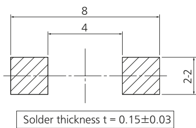
PWB land pattern for reference
