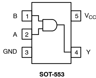
Figure 2. Pinout (Top View)
