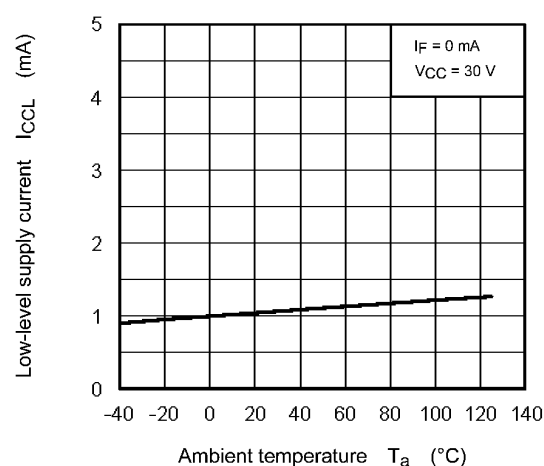
Fig. 13.2.5 I_{CCL} - T_a
