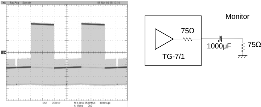
c) 1000 \mu\text{F} + 150 \Omega sag waveform (TV Test Signal Generator Sibasoku TG-7/1 output, H-bar)
