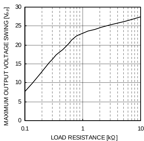
Fig.5 Maximum Output Voltage Swing - Load Resistance (VCC/VEE=+15V/-15V, T a =25°C)
