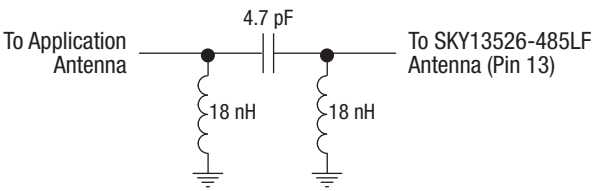
ESD Circuit 1
