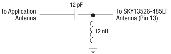
ESD Circuit 2
