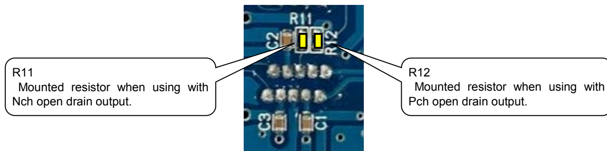
Figure 3 R11,R12 land
