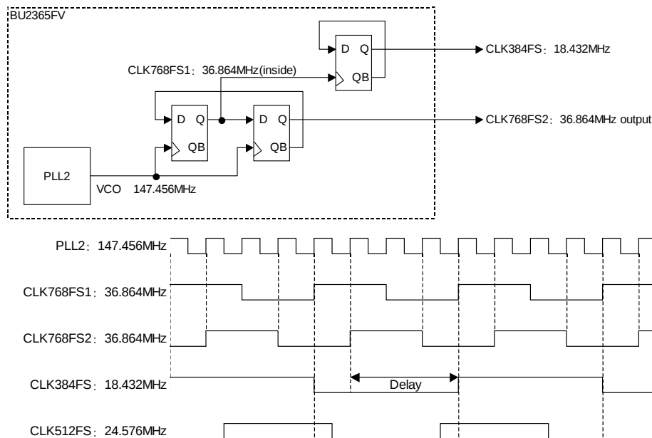
Fig.79 Audio Clock Output Circuit Configuration and Timing Chart
