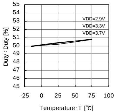
Fig.58 27MHz VCXO Temperature—Duty
