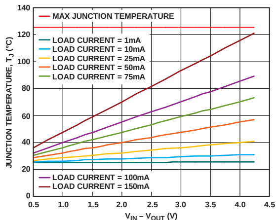
Figure 30. 500 mm 2 of PCB Copper, T_A = 25^\circ\text{C}
