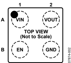
Figure 4. Pin Configuration
