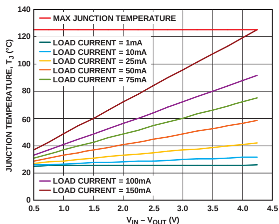
Figure 31. 100 mm 2 of PCB Copper, T_A = 25^\circ\text{C}
