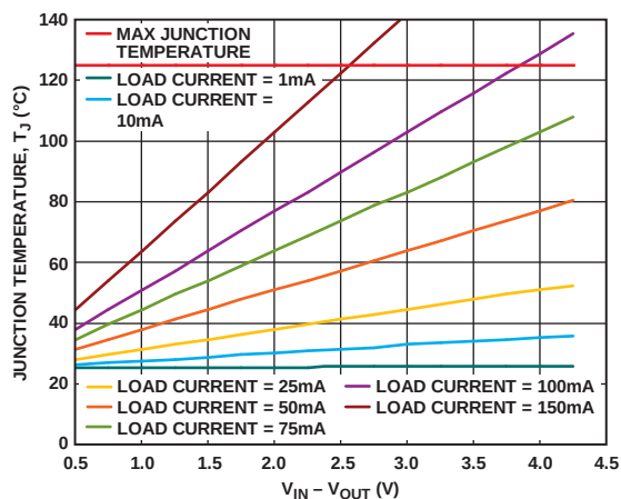
Figure 32. 0 mm 2 of PCB Copper, T_A = 25^\circ\text{C}
