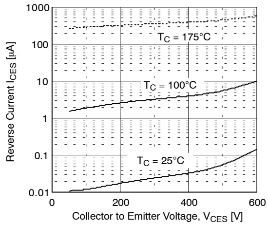
Figure 22. Reverse Current
