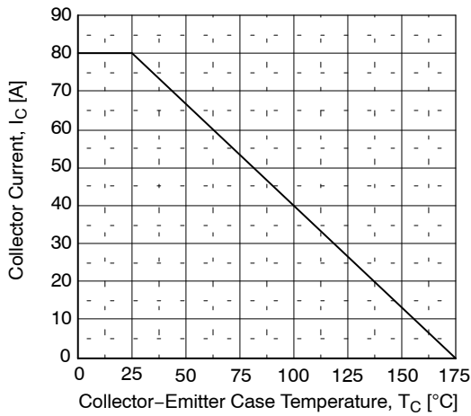
Figure 19. Current Derating
