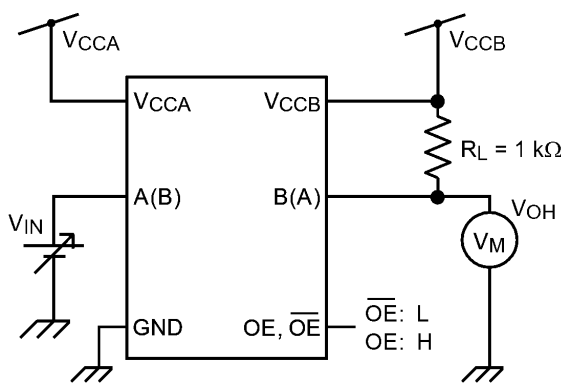
Fig. 15.1 Test Circuit
