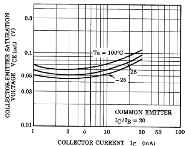
Fig. 10.22 RN1304 V_{CE(sat)}-I_C
