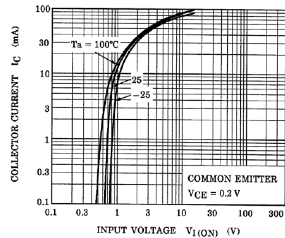
Fig. 10.5 RN1305 I_C - V_{I(ON)}
