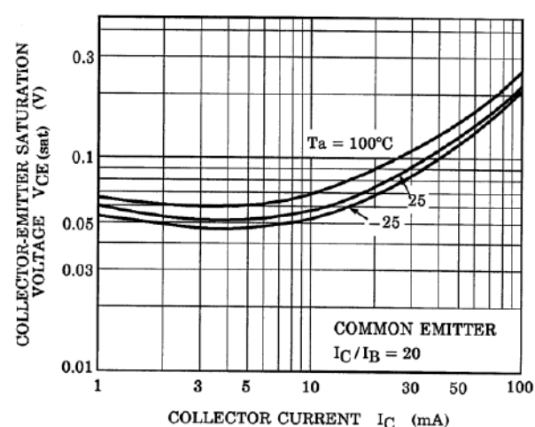
Fig. 10.23 RN1305 V_{CE(sat)}-I_C
