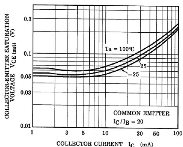
Fig. 10.24 RN1306 V_{CE(sat)}-I_C
