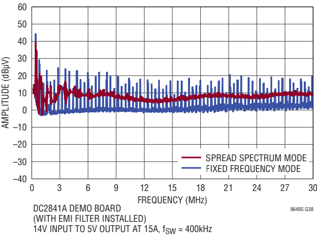
Conducted EMI Performance
