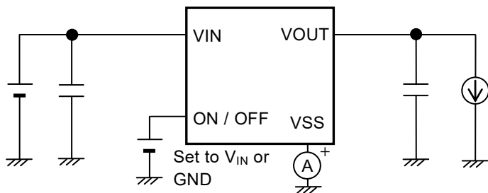
Figure 6 Test Circuit 2
