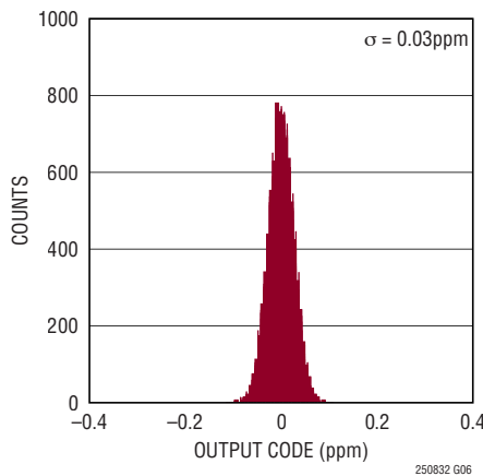
DC Histogram, DF = 4096
