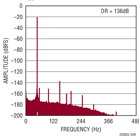
128k Point FFT f_{SAMPL} = 1\text{Msps} , f_{IN} = 50\text{Hz} , DF = 1024
