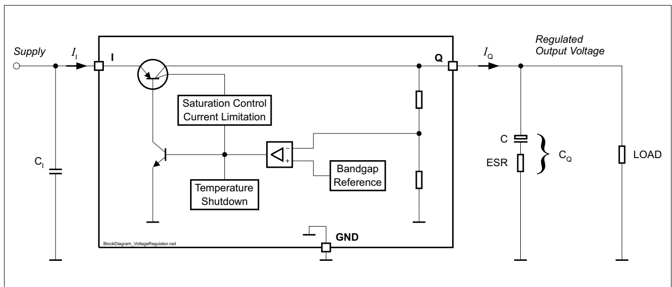
Figure 3 Voltage regulator
