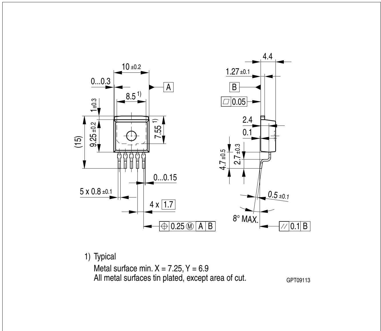
Figure 8 PG-T0263-5 1)
