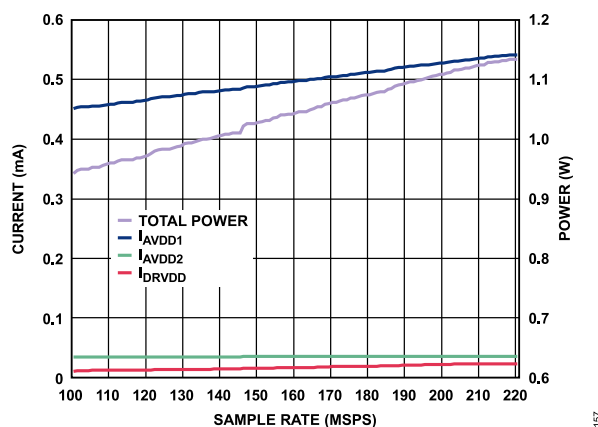
Figure 62. Supply Current vs. f_{\text{SAMPLE}} for f_{\text{IN}} = 5 \text{ MHz} , AD9467-200
