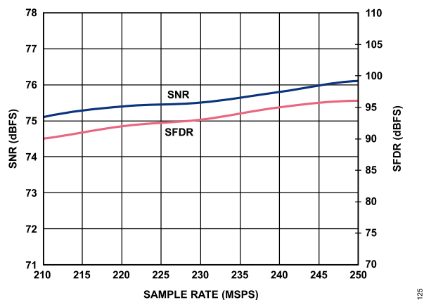
Figure 23. SNR/SFDR vs. f_{\text{SAMPLE}} , f_{\text{IN}} = 97.3 \text{ MHz} , 2.5 V p-p FS, AD9467-250
