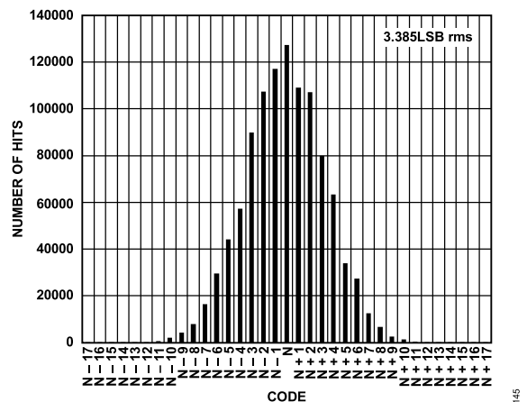
Figure 45. Input-Referred Noise Histogram, 2.5 V p-p FS, AD9467-250
