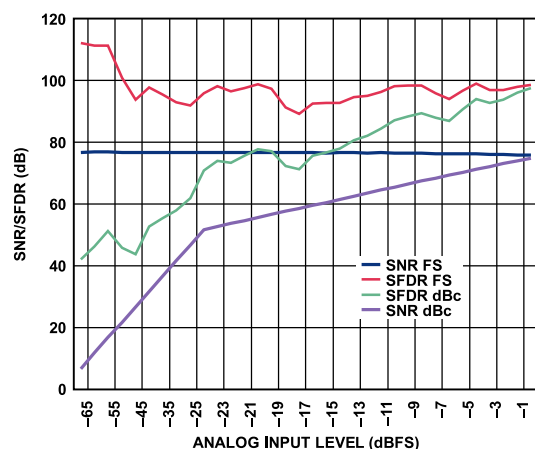
Figure 32. SNR/SFDR vs. Analog Input Level, f_{IN} = 97.3 MHz, 2.5 V p-p FS, AD9467-200
