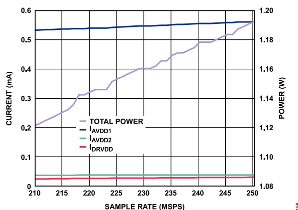
Figure 63. Supply Current vs. f_{\text{SAMPLE}} for f_{\text{IN}} = 5 \text{ MHz} , AD9467-250
