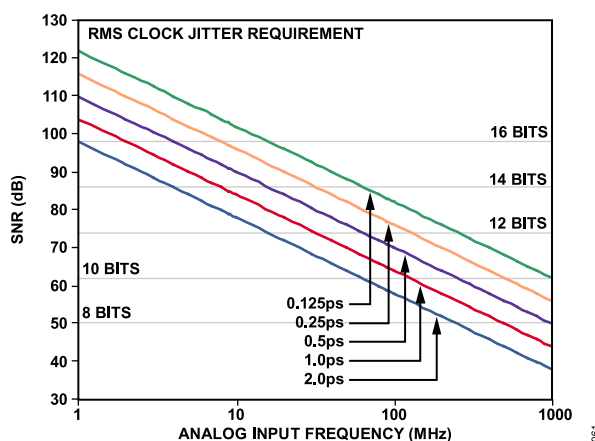
Figure 61. Ideal SNR vs. Input Frequency and Jitter
