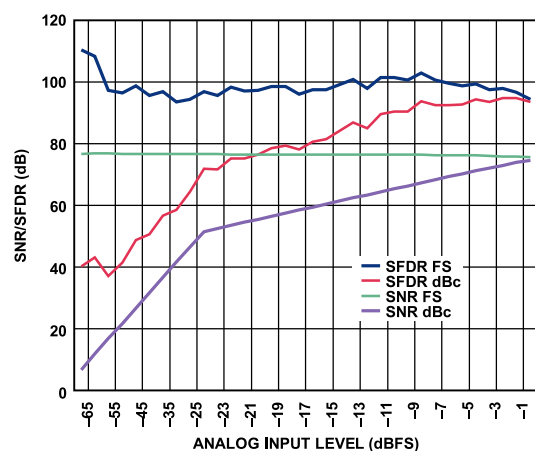
Figure 33. SNR/SFDR vs. Analog Input Level, f_{IN} = 97.3 MHz, 2.5 V p-p FS, AD9467-250
