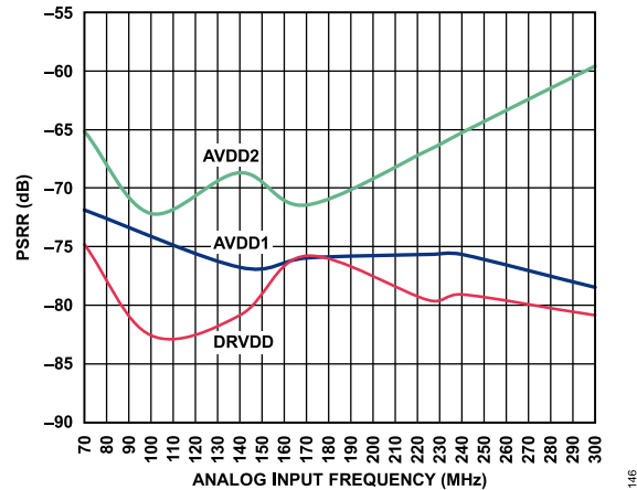
Figure 46. Power Supply Rejection (PSR), AD9467-250
