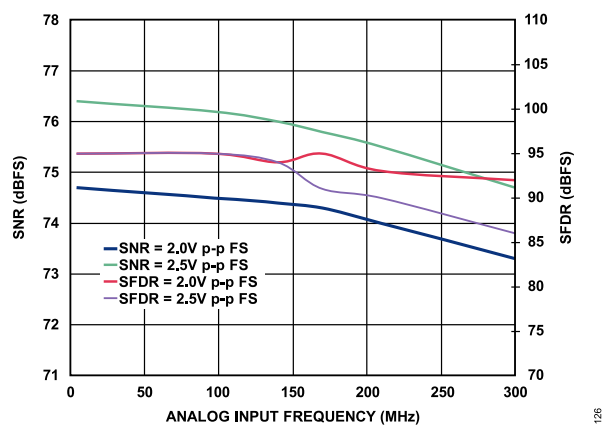
Figure 26. SNR/SFDR vs. f_{\text{IN}} , 2.0/2.5 V p-p FS, AD9467-200
