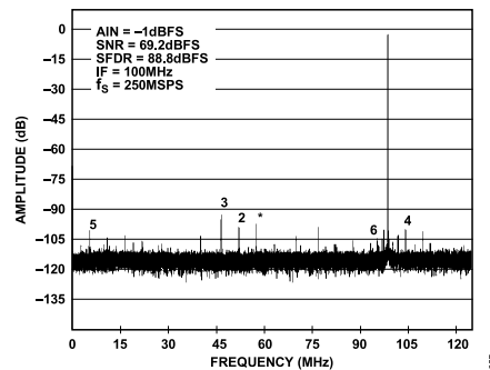
Figure 57. Single-Tone FFT Performance Plot Using the ADL5201 VGA, Gain = 20 dB, and the AD9467-250
