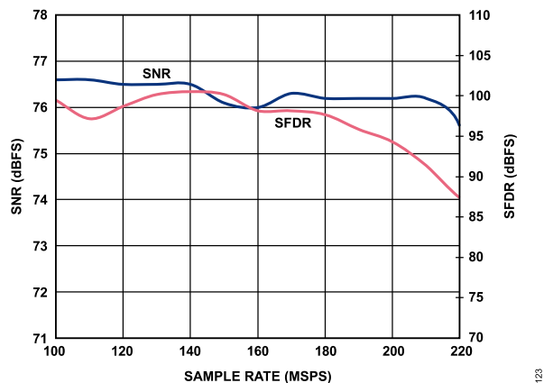
Figure 22. SNR/SFDR vs. f_{\text{SAMPLE}} , f_{\text{IN}} = 97.3 \text{ MHz} , 2.5 V p-p FS, AD9467-200
