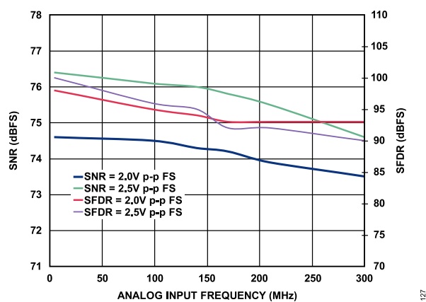
Figure 27. SNR/SFDR vs. f_{\text{IN}} , 2.0/2.5 V p-p FS, AD9467-250
