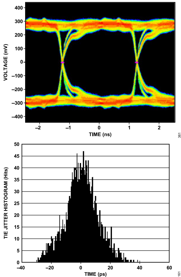
Figure 66. Data Eye for LVDS Outputs in ANSI-644 Mode with 18-Inch Trace Lengths on Standard FR-4, AD9467-250
