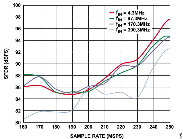
Figure 25. SFDR vs. f_{\text{SAMPLE}} , 2.5 V p-p FS, AD9467-250
