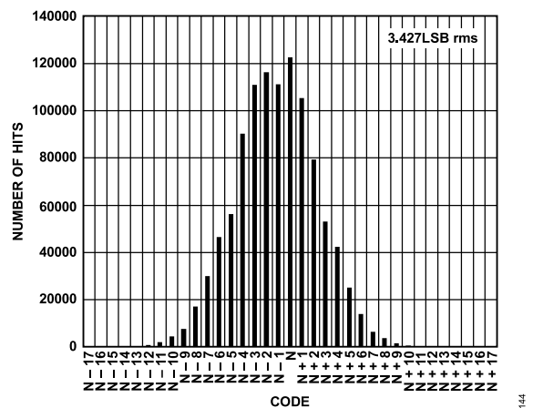
Figure 44. Input-Referred Noise Histogram, 2.5 V p-p FS, AD9467-200
