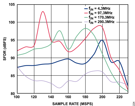
Figure 24. SFDR vs. f_{\text{SAMPLE}} , 2.5 V p-p FS, AD9467-200
