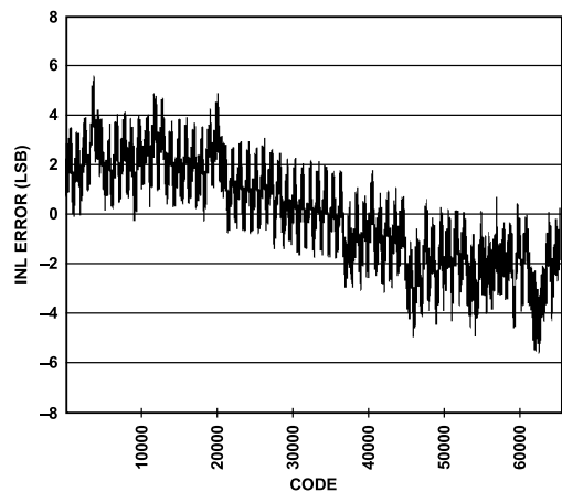
Figure 38. INL, f_{IN} = 4.3 MHz, 2.5 V p-p FS, AD9467-250
