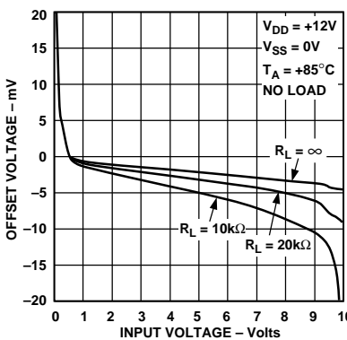
Figure 8. Offset Voltage vs. Input Voltage
