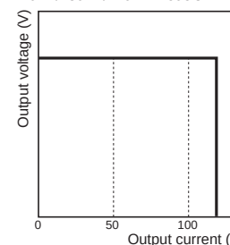
120-W/180-W/240-W Models
