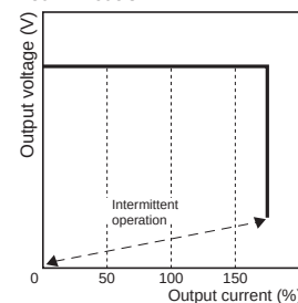
480-W Models
