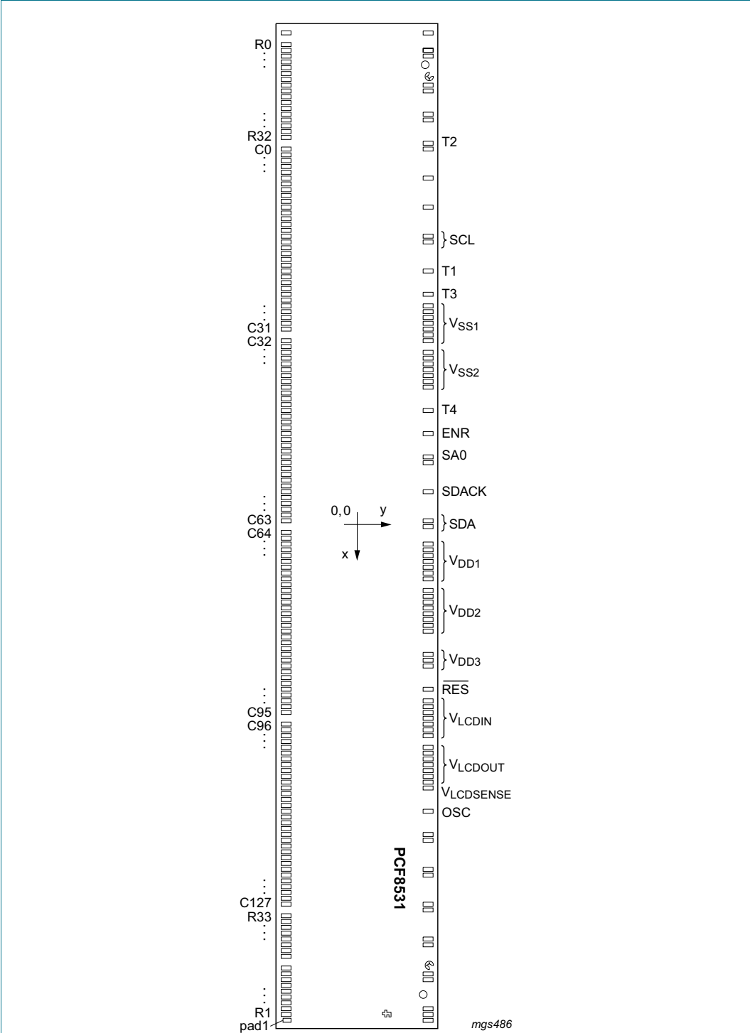
Viewed from active side. The positioning of the bonding pads is not to scale. Fig 2. Bonding pad location for PCF8531
