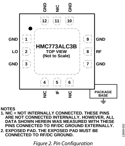
Figure 2. Pin Configuration
