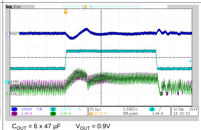
Figure 26. Typical Operation (PSM)
