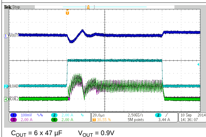
Figure 25. Typical Operation (PWM)
