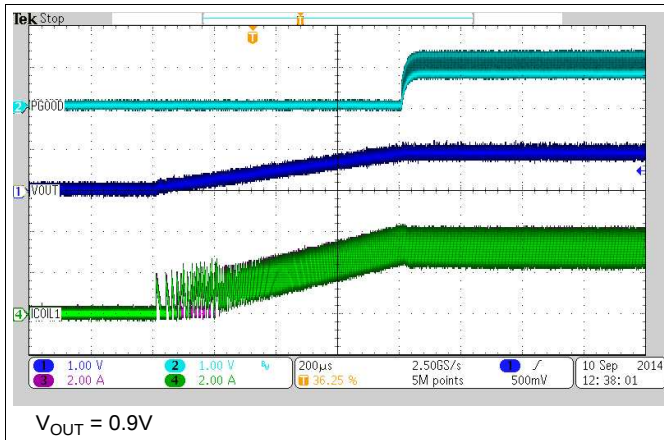
Figure 23. Startup into 0.135 \Omega (6.6 A)
