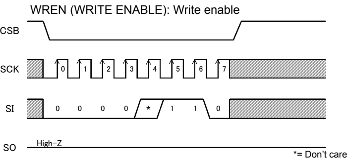
Figure 35. Write enable command
