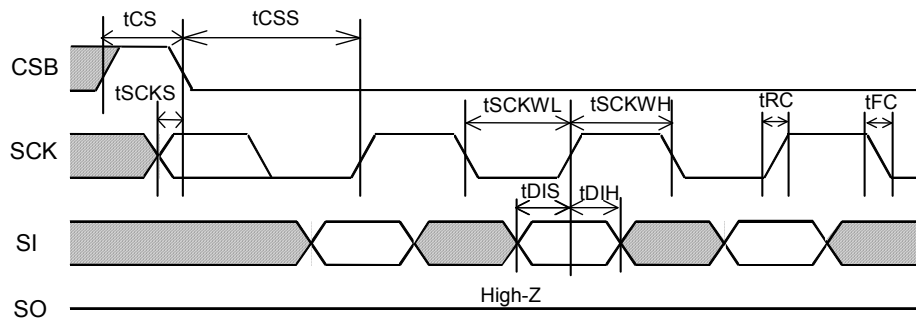
Figure 2. Input timing
