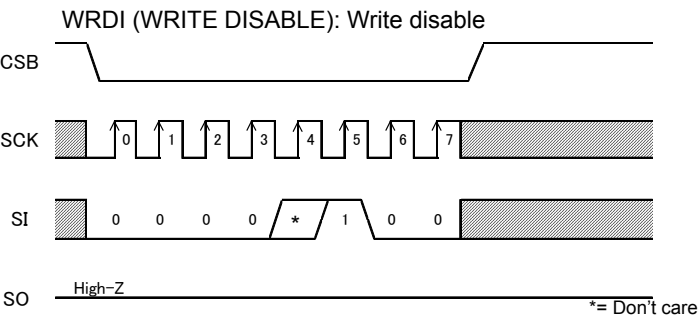
Figure 36. Write disable
