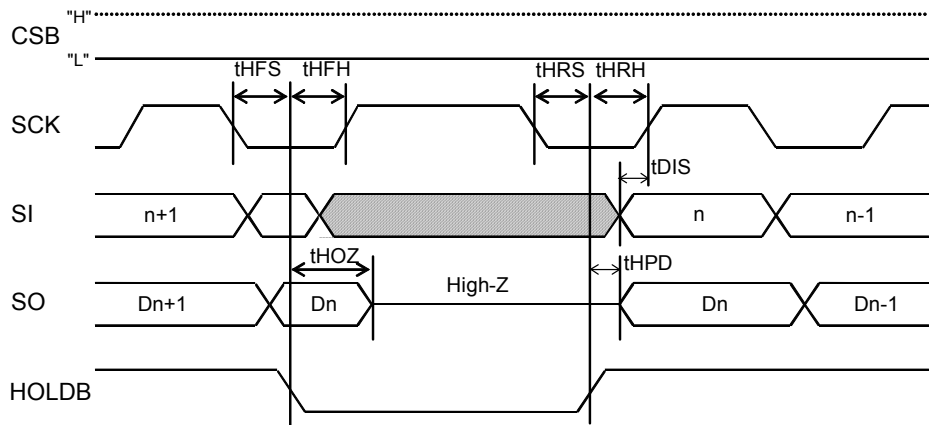
Figure 4. HOLD timing
